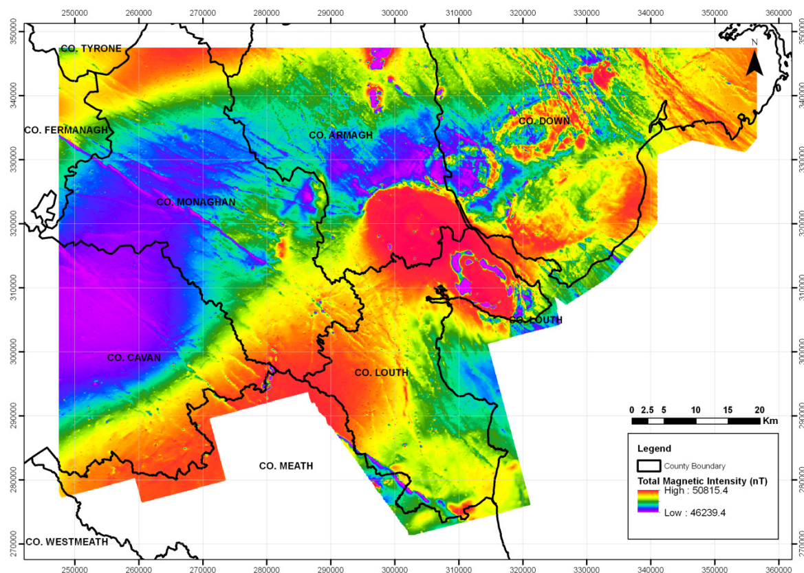
Figure 4.1: Total Magnetic Intensity data prior to processing.
