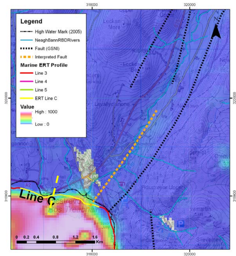
Figure 6.21: EM 12 kHz frequency showing fault locations and marine ERT survey Line C.
