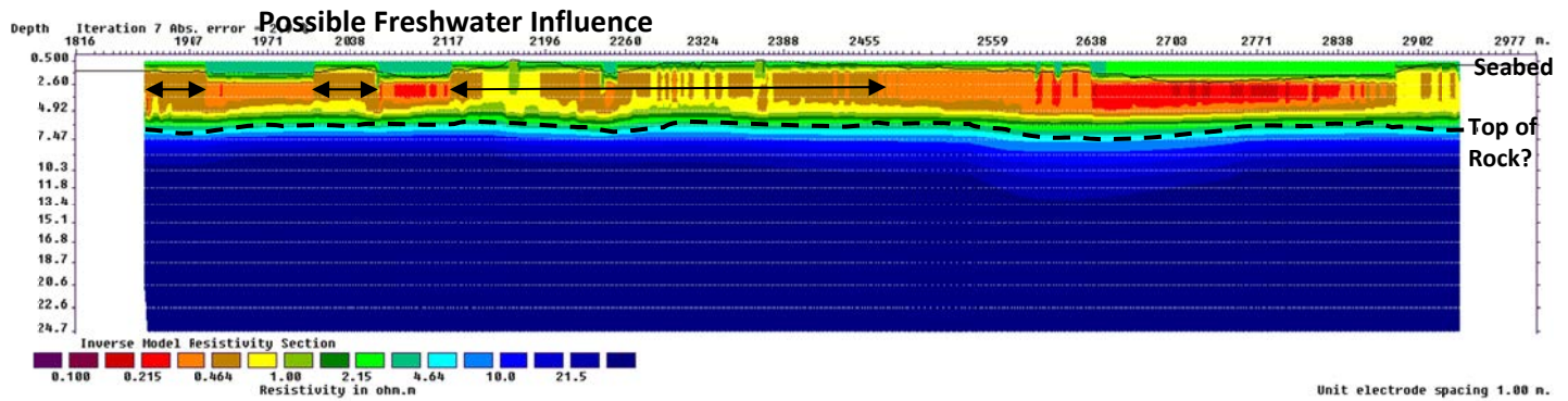
Figure 6.20: Marine ERT Line 5 along western shoreline of Carlingford Lough. Higher resistivity sediments indicated by black arrows. Dashed line indicates probable top of rock.
