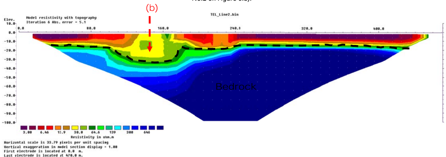
Figure 6.12: ERT Line 2.
