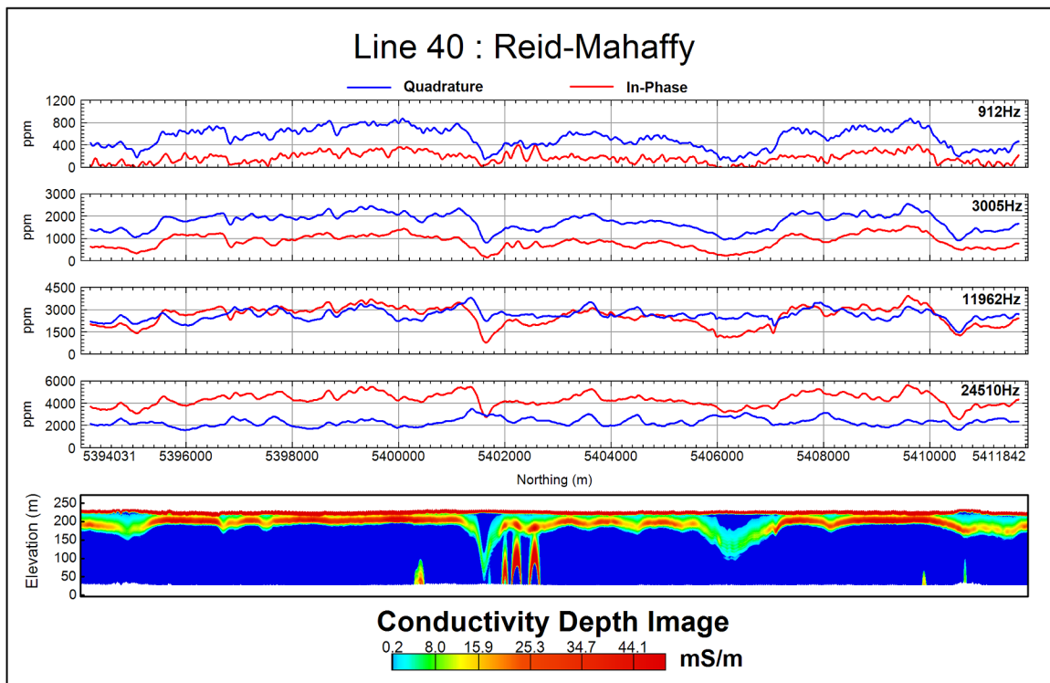
Test line over the Reid-Mahaffy test site in Ontario showcasing all electromagnetic components in profile plus CDI generated from all SGFEM frequencies. The targets of interest can be seen in the centre of the CDI along with the overburden across the entire length of the line.
